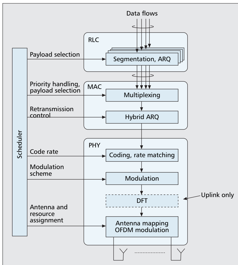
■ Figure 1. LTE protocol structure (simplified).
