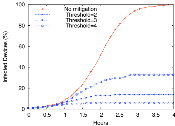
Fig. 6. Infection over time using proximity-based signature dissemination.
