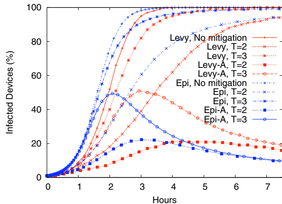
Fig. 5. Effects of local detection on malware propagation, evaluated both with Levy walk simulations and the epidemic model.
