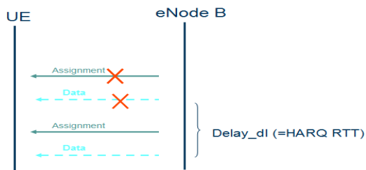
Figure 3. Error upon transmission of DL assignment.
