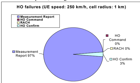
Figure 5. Percentage of failures occurring upon transmission of the different HO involved messages; UE speed 250 km/h and cell radius 1 km.
