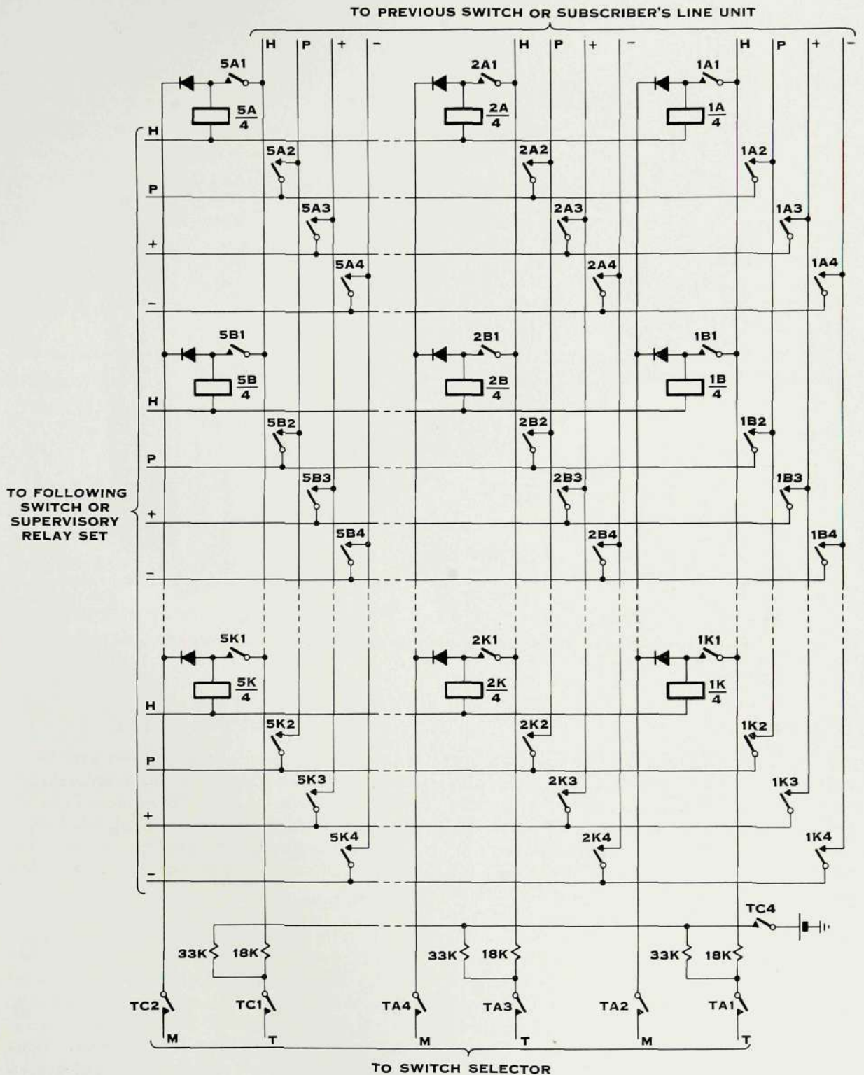
Figure 10—Cross-Point Switch. This diagram shows the wiring multiples consisting of a speech pair (+ and -) and control wires (H and P). The relay contacts enable any vertical and horizontal multiple to be connected together. The test wires (T) are the input leads to the switch selector; the mark wires (M) are the output leads from it
