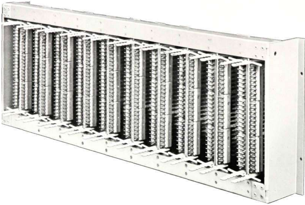
Figure 23—A removable shelf unit of the DSU Equipment. (Rear view showing wiring tags.) This unit can be wired before assembly into the rack if desired
