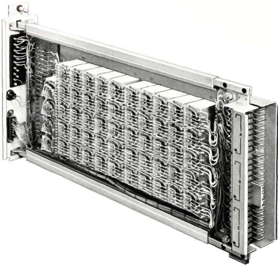
Figure 11—C Switch. Three-quarter rear view showing horizontal wiring multiples
