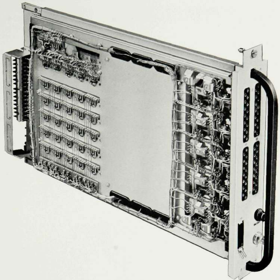
Figure 8— Subscribers' Line Unit and 5 × 5 'A' Switch. The Line Unit contains five line circuits
