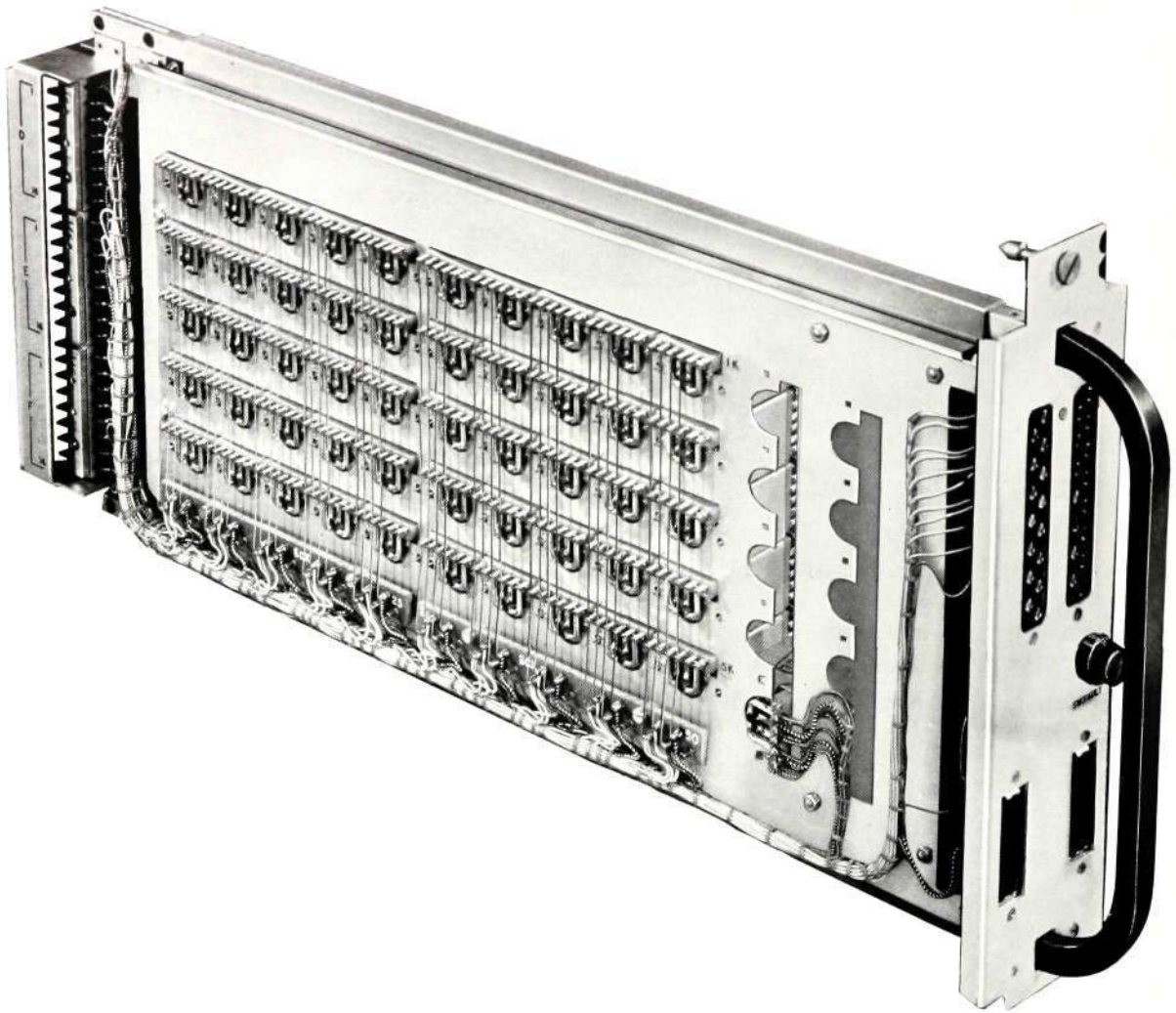
Figure 5—B switch (5 × 10). Two of these units are used to form a 10 × 10 switch. The single relay near the front panel is the Alarm Relay
