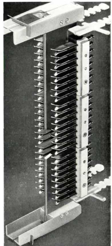
Figure 22—The Jack Assembly of the DSU Equipment. The tapered mortise in the vertical plate facilitates accurate location of plug and jack
