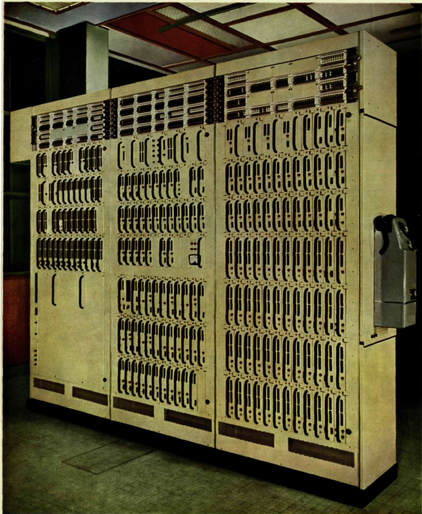
The prototype Pentex Exchange ready for installation at Peterborough
