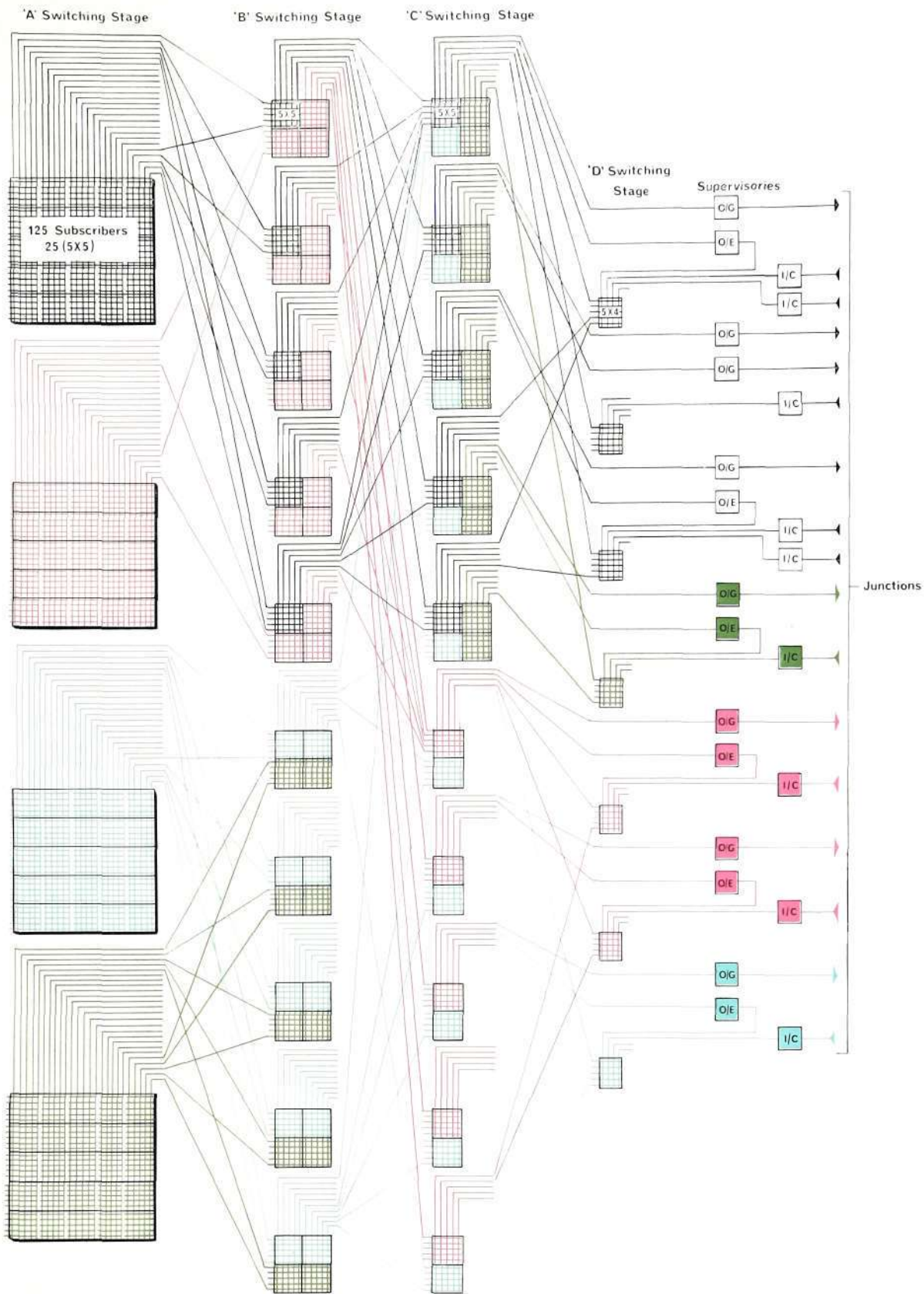
Figure 6—Trunks diagram
