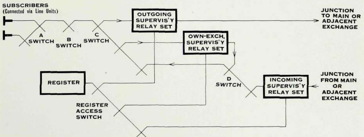
Figure 2—Simplified block diagram of a Pentex Exchange
