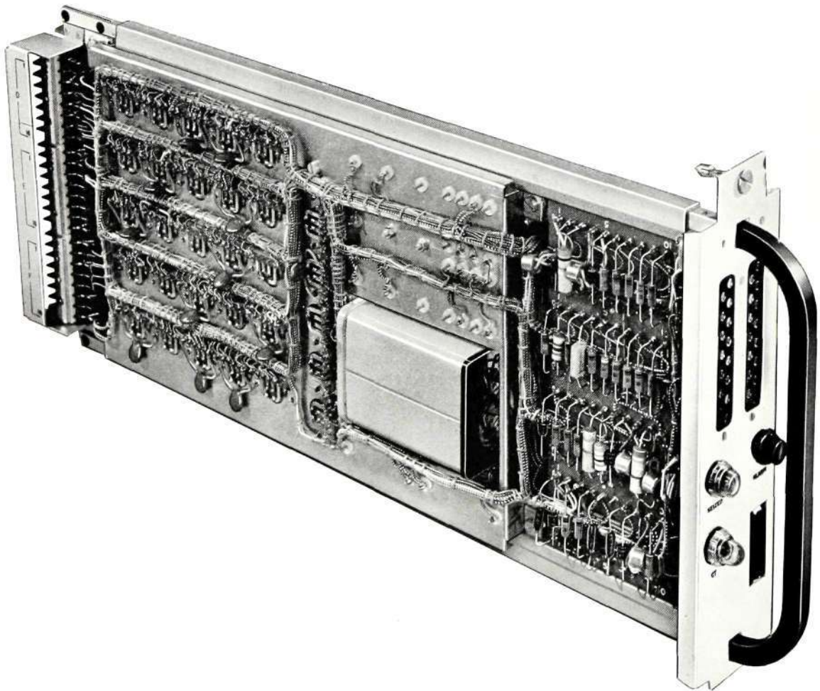
Figure 14—Incoming Supervisory Relay Set. This view shows how larger components can be accommodated, by through-panel mounting
