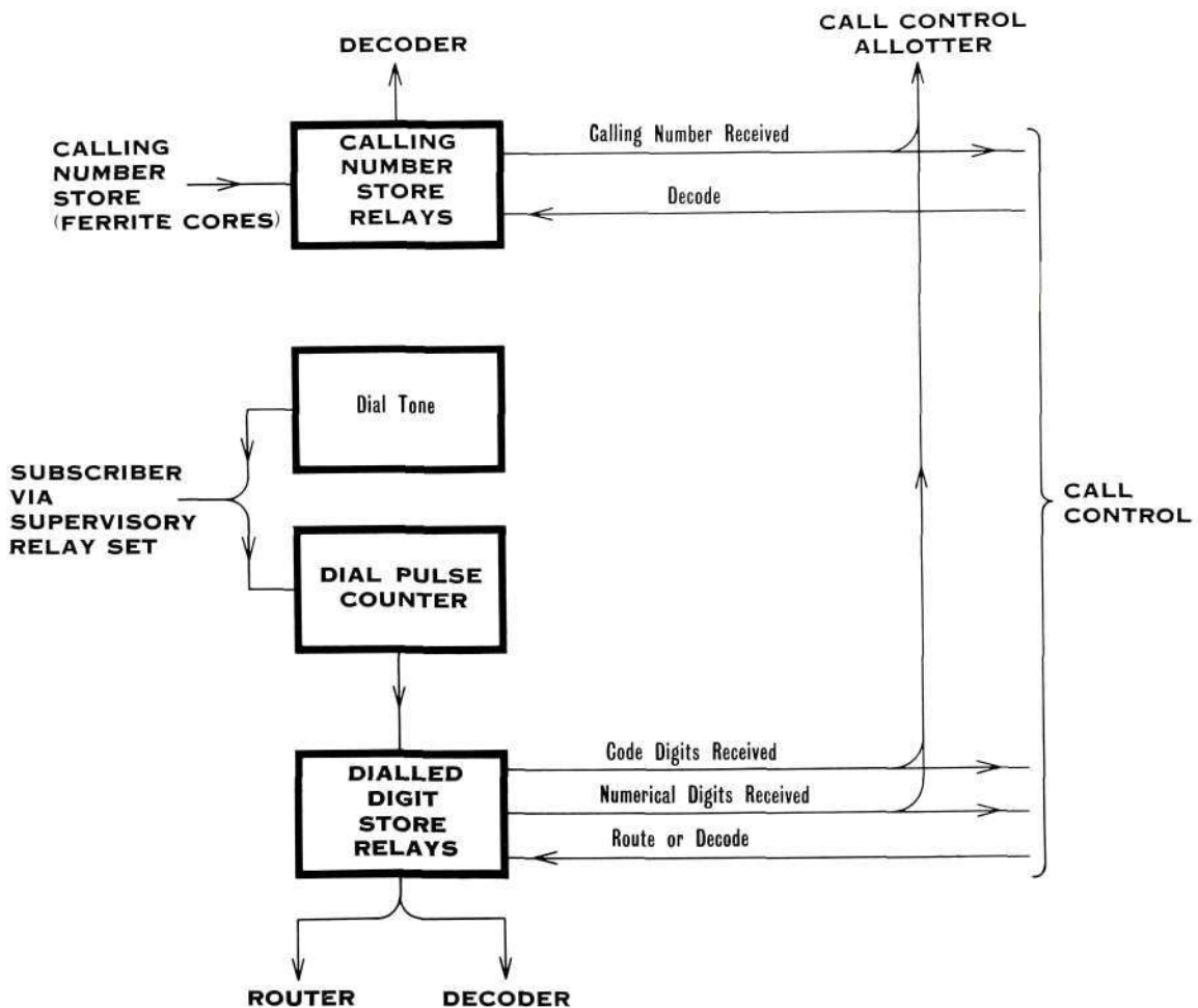
Figure 12—Register block diagram, showing circuits and signals used in the storage of numbers
