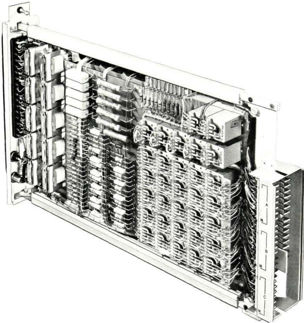
Figure 18—Subscribers' Line Unit and 5 × 5 'A' Switch. (Three-quarter rear view)
