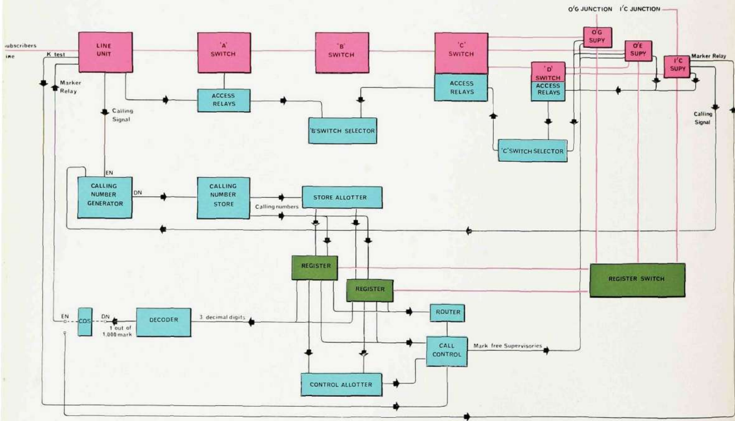
Figure 7—Control diagram
