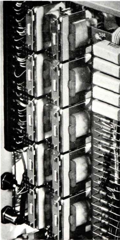
Figure 17—The front end of the Subscribers' Line Unit, showing two Strip Relays (Type 12). These relays, developed by E.T.L., consist of five independent relays on a common yoke, providing one L and one K relay for each of the five Subscribers' Line Circuits
