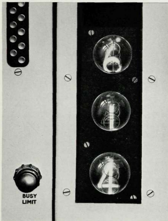
Figure 4—Number Display Unit. The self-luminous Digitrons enable the digits of the calling or called number to be readily observed
