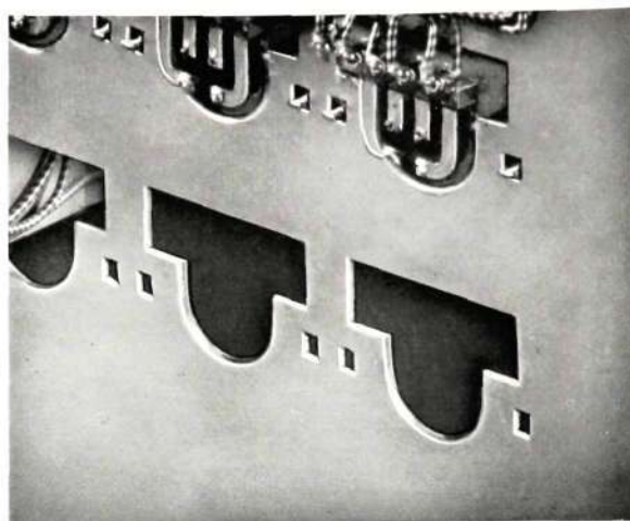
Figure 19—Part of the Register, showing holes blanked-out of the mounting plate. Fixing the reed relays in this way enables connections to be made from each side of the mounting plate
