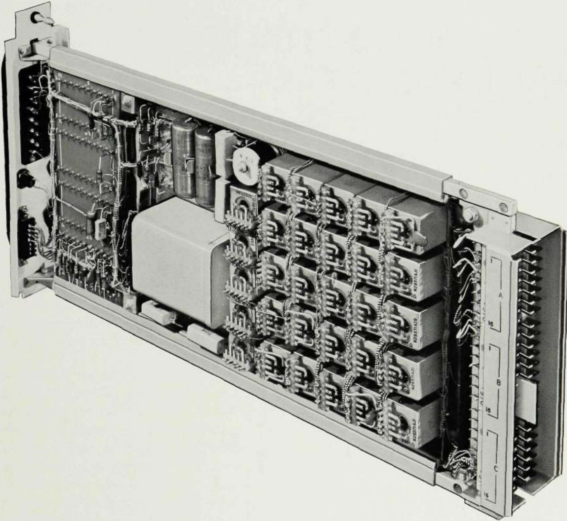
Figure 15—Incoming Supervisory Relay Set. (Three-quarter rear view)
