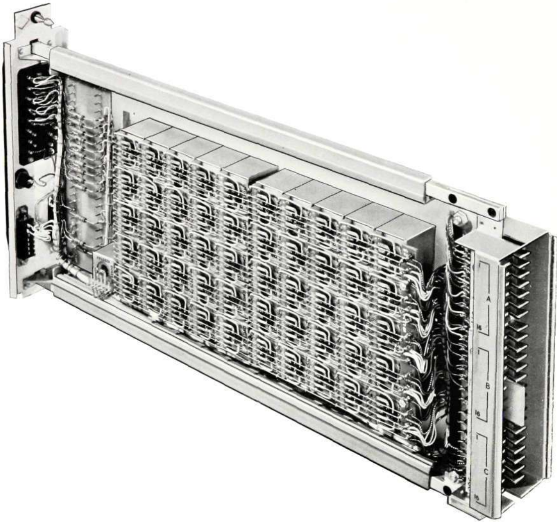
Figure 13—B Switch (5 × 10), showing horizontal wiring multiples
