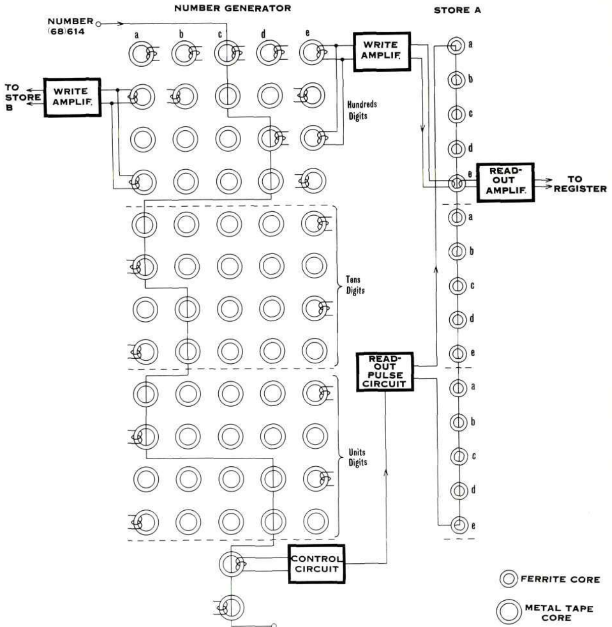
Figure 16—Calling Number Generator and Store. The subscriber's full number is not generated since the first two digits (68) are the exchange code digits common to all subscribers on that exchange
