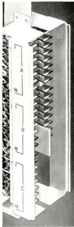
Figure 21—Jack-plug at the rear of a jack-in panel. This view shows the metal tongue which engages with a mortise on the jack-plate
