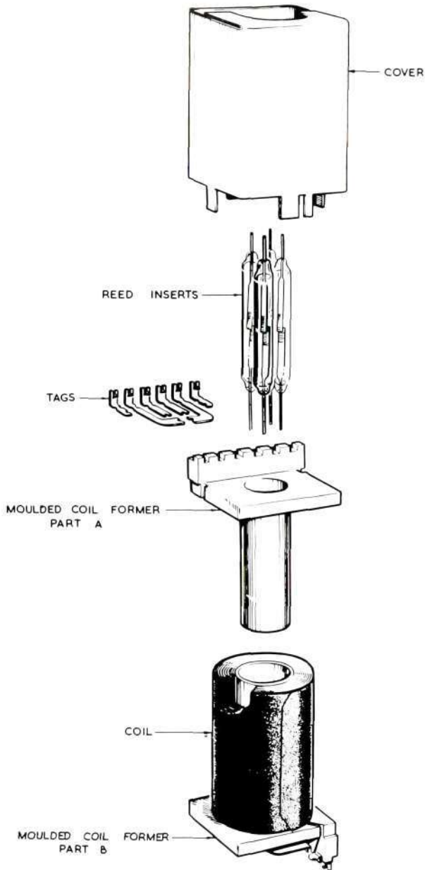
Figure 25—Constructional details of the Reed Relay. The cover provides a magnetic return path for the reed inserts and also acts as a magnetic screen
