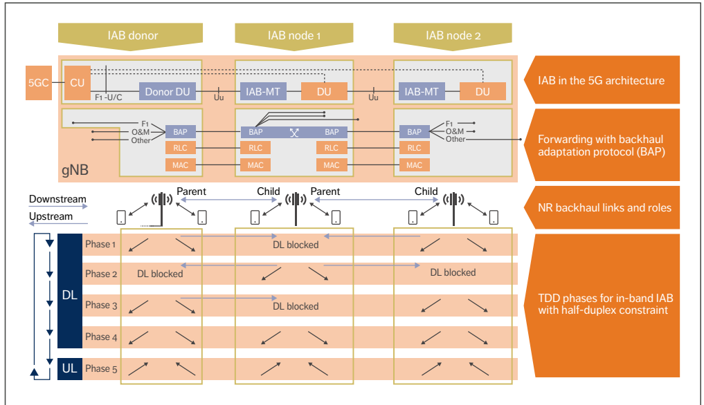
Figure 2 The 3GPP IAB concept
