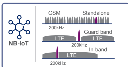
Figure 13: NB-IoT deployment.
