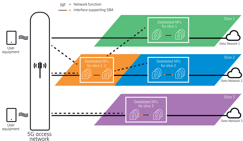
Figure 2: Simplified 3GPP 5G architecture
